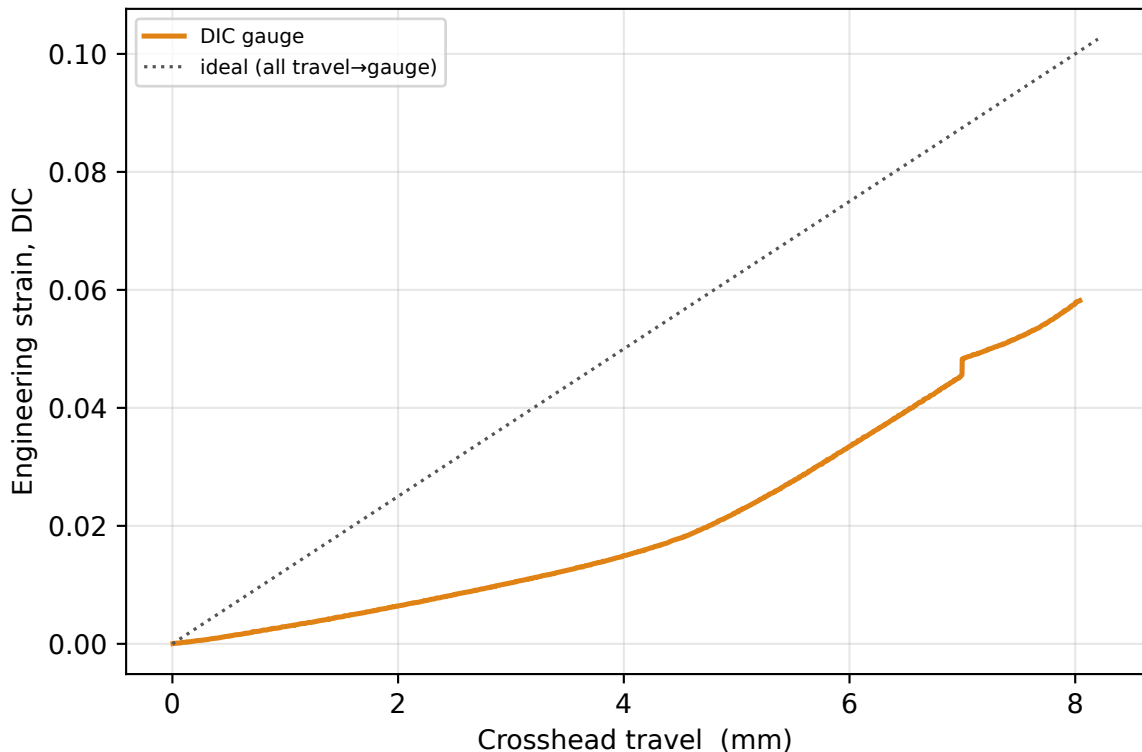
DIC strain vs crosshead — the compliance gap
